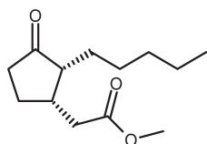
Cyclopentaneacetic acid, 3-oxo-2-pentyl-, methyl ester
